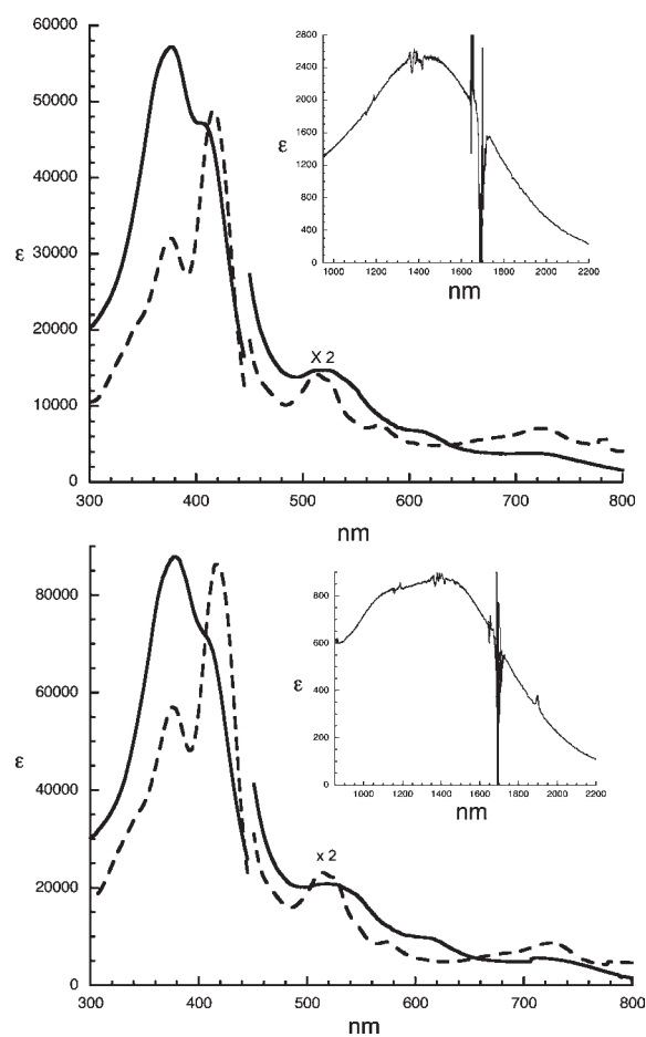
Figure 1. UV-vis spectra of [Fe(TEtP*)(Cl)] (dashed line) and [Fe(TEtP*)(Cl)]SbCl 6 (solid line) (Top), and [Fe(TPrP*)(Cl)] (dashed line) and [Fe(TPrP*)(Cl)]SbCl 6 (solid line) (Bottom) in CH 2 Cl 2 solution. Insets in both sets of spectra display the near-IR band of [Fe(TEtP*)(Cl)]SbCl 6 (top) and [Fe(TPrP*)(Cl)]SbCl 6 (bottom).
