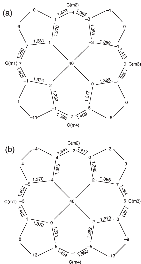
Figure 6. Formal diagrams of the porphinato core displaying perpendicular displacements, in units of 0.01 Å, of the core atoms from the 24-atom mean plane. Also entered on the diagrams are the values of the individual bond distances in the inner 16-membered rings. Note the alternating short–long pattern of the N–C a and C a –C m bond distances. [Fe(TETP • )(Cl)]SbCl 6 (top), [Fe(TPrP • )(Cl)]SbCl 6 (bottom).
