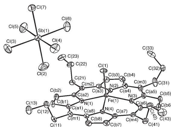
Figure 3. ORTEP diagram of [Fe(TPrP*)(Cl)]SbCl 6 displaying the atom labeling scheme. Thermal ellipsoids of all atoms are contoured at the 50% probability level. Hydrogen atoms have been omitted for clarity.
