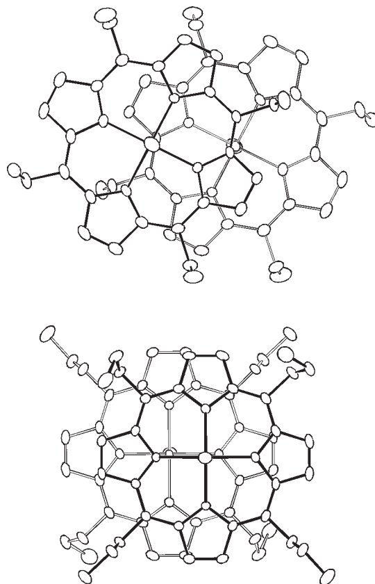
Figure 5. Top-views of the dimeric units of [Fe(TeTP*)(Cl)] + (top) and [Fe(TPrP*)(Cl)] + (bottom). (50% probability ellipsoids).
