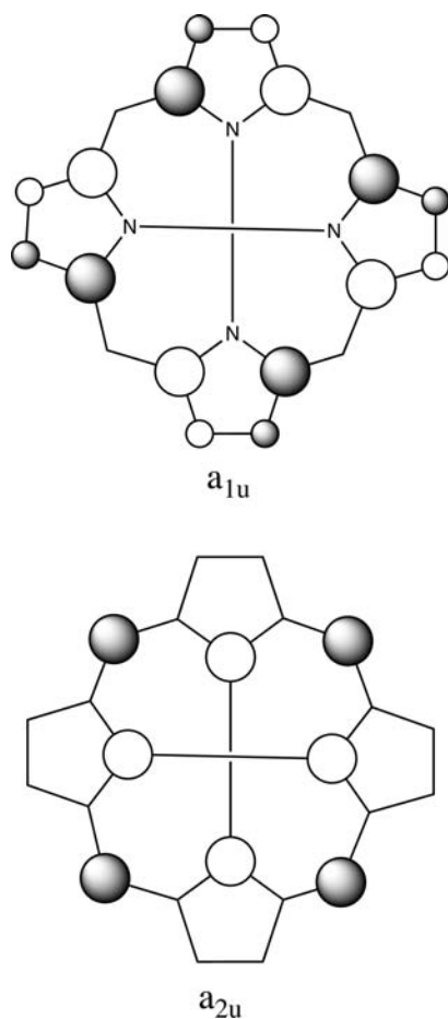
Scheme 1. Plots of HOMOs of a_{1u} and a_{2u} Symmetry a
