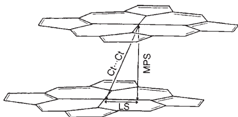
Scheme 2. Diagram Illustrating Structural Features Found in Cofacial Porphyrin Dimers a
