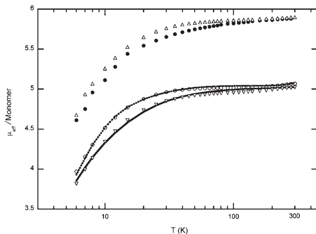
Figure 7. Comparison of observed and calculated values of \mu_{\text{eff}}/\text{monomer} vs T for [\text{Fe}-(\text{TETp}^*)(\text{Cl})]\text{SbCl}_6 ( \circ ) and [\text{Fe}(\text{TPrP}^*)(\text{Cl})]\text{SbCl}_6 ( \nabla ). The lines (solid or dashed) are model calculations assuming pairwise spin coupling. The fit parameters used are given in Table 3. Also shown in the figure are the T -dependent magnetic susceptibilities for the precursors [\text{Fe}(\text{TPrP})(\text{Cl})] ( \bullet ) and [\text{Fe}(\text{TETp})(\text{Cl})] ( \Delta ) that have been described previously. 11
