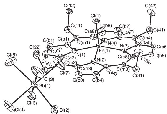
Figure 2. ORTEP diagram of [Fe(TeTP*)(Cl)]SbCl 6 displaying the atom labeling scheme. Thermal ellipsoids of all atoms are contoured at the 50% probability level. Hydrogen atoms have been omitted for clarity.
